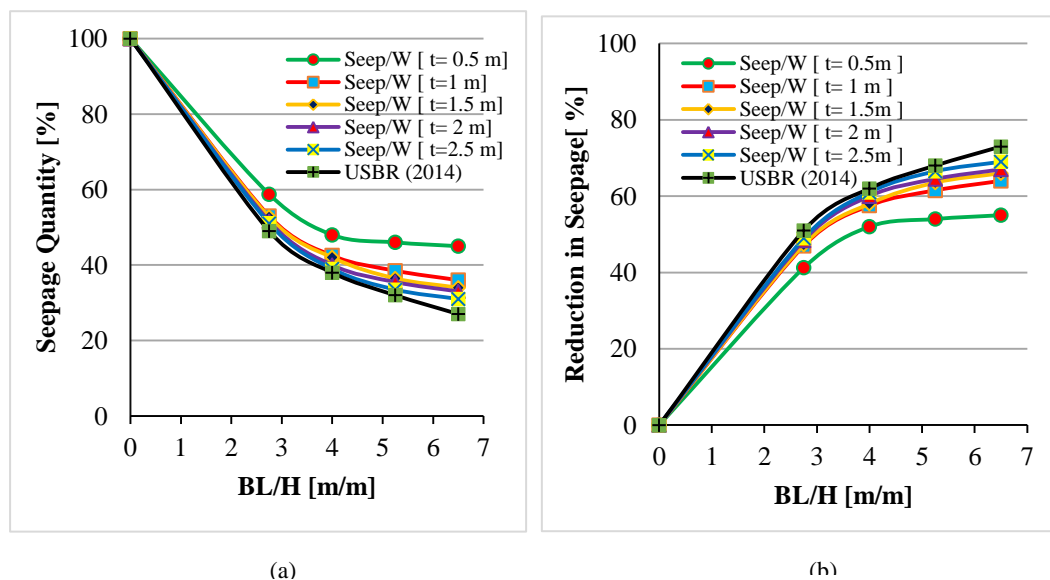
Figure 2: The relationship between the percentage of (a) seepage quantity and (b) seepage reduction with the ratio of blanket length to the water head ( BL/H ) for different blanket thicknesses compared to the curve plotted by (USBR (2014))
