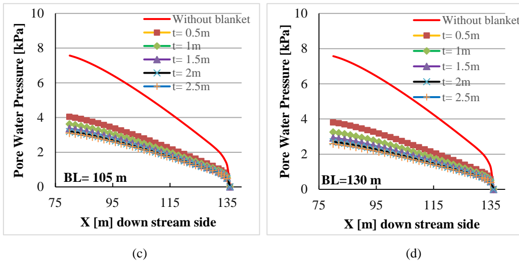
Figure 4: The distribution of pore water pressure at the downstream side directly under the embankment due to the effects of the variation of blanket thickness and blanket length (a) BL= 55m, (b) BL= 80m, (c) BL= 105m, and (d) BL= 130 m
