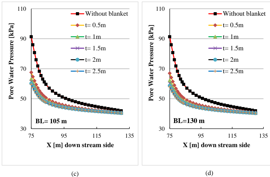
Figure 5: The distribution of pore water pressure at the downstream side four meters under the embankment due to the effects of the variation of blanket thickness and blanket length (a) BL= 55m, (b) BL= 80m, (c) BL= 105m, and (d) BL= 130 m
