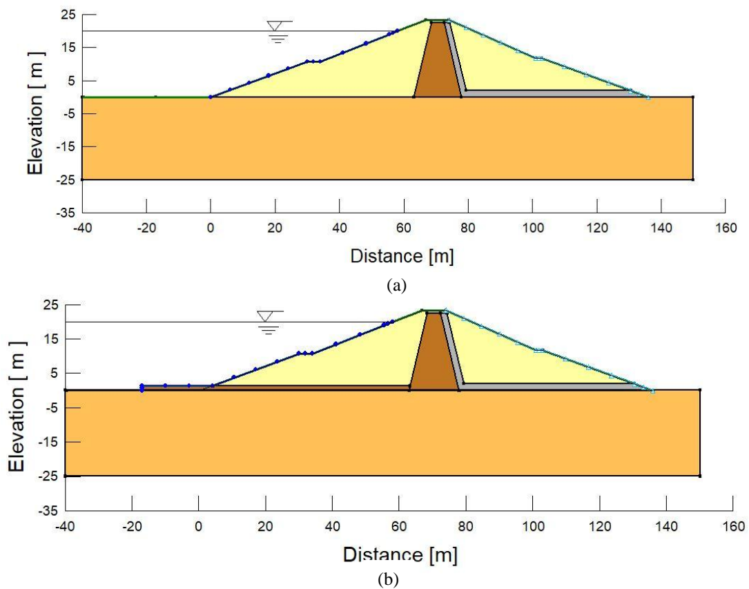
Figure 1: Cross section of Shiwashok earth dam used in this study (a) without clay blanket (b) With clay blanket
