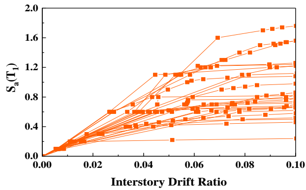
Figure 5: IDA curve of the 6-story structure having soil D including near field pulse like records.
