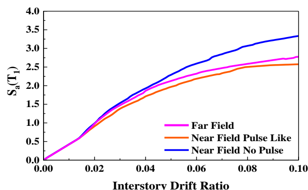
Figure 7: Med_{IDA} of the 2-story structure having soil D including three record subsets.
